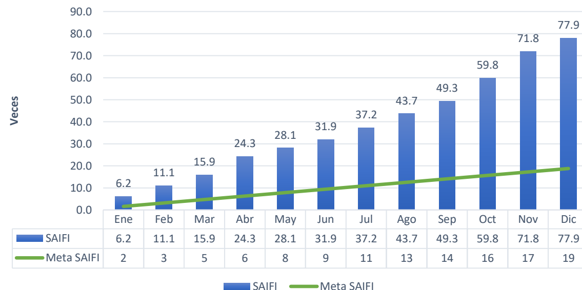
SAIFI 2019
