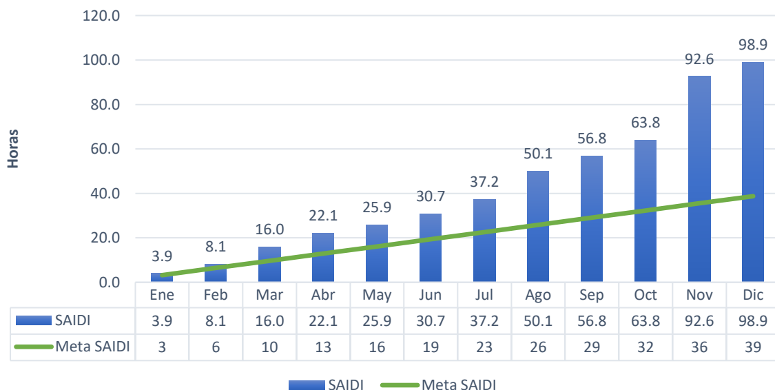
SAIDI 2019
